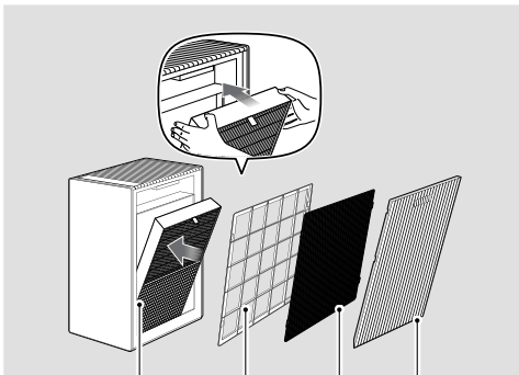
Max2 filter Pre-filter frame Pre-filter Cover
